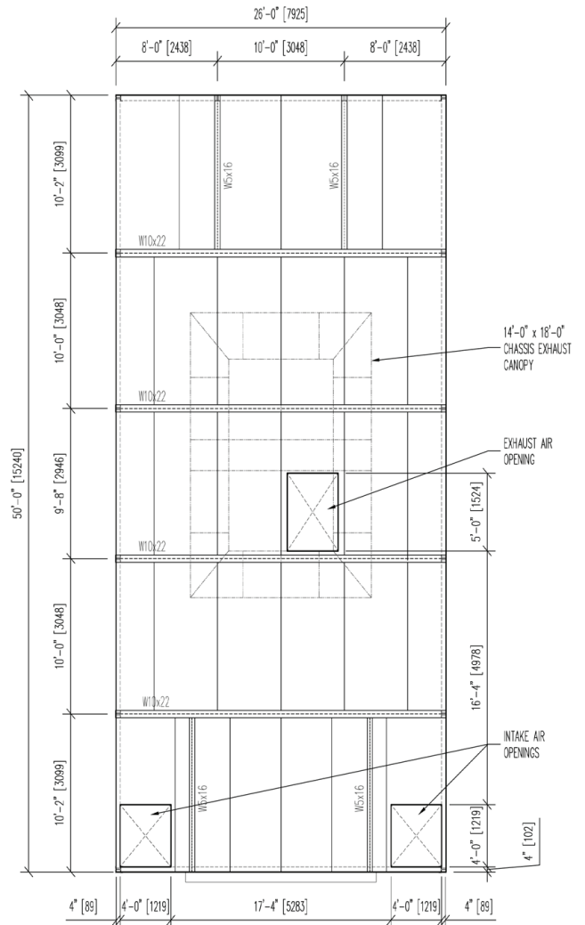
CHASSIS TEST CELL - ROOF PLAN
