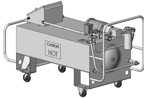
DK0008 Oil Preheat and Supply Cart shown
