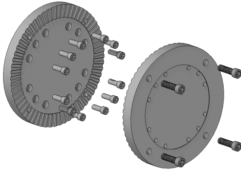
1014164 1810 Quick Connect Kit shown
